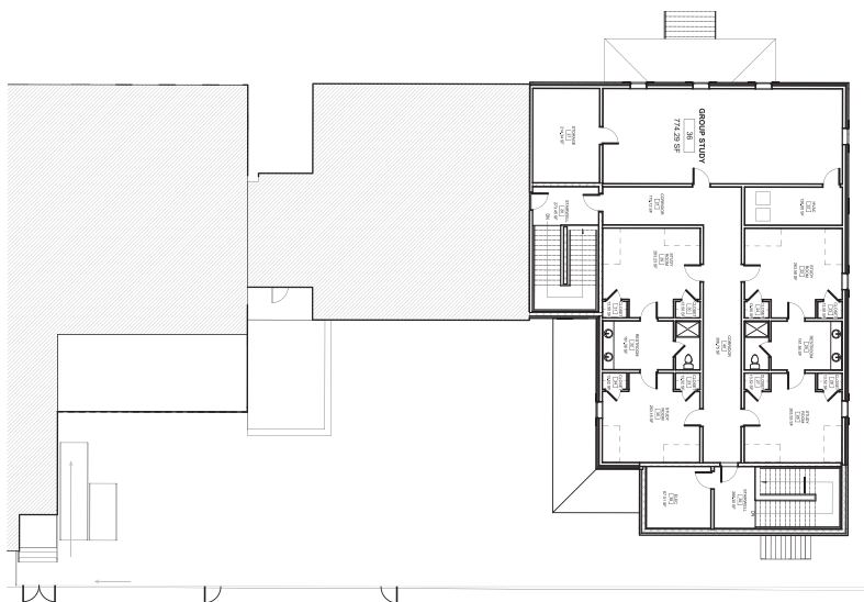
SECOND FLOOR 1/8" = 1'-0"
